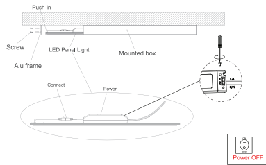
C: Push the fixture into the mounted box and secure the Alu frame.
