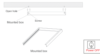
B: Put the mounted box on the wall.
